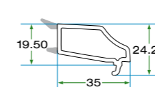
K 6007 DEKORATİF ÇANTALI TEK CAM ÇİTASI K 6007 DECORATIVE SINGLE GLAZING BEAD WITH GRAY GASKET
