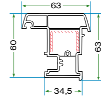
K 6021 HAREKETLİ ORTA KAYIT PROFİLİ K 6021 MOVABLE MULLION PROFILE
