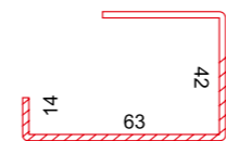
KAPI DESTEK SAÇI DOOR STEEL REINFORCEMENT
