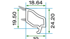
K 6006 DEKORATİF ÇİFT CAM ÇİTASI K 6006 DECORATIVE DOUBLE GLAZING BEAD WITH GRAY GASKET
