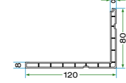
K 6010 80x120 PERVAZ PROFİLİ K 6010 80 x 120 BORDER PROFILE
