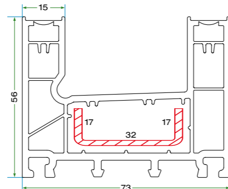
KPS 6208 ÇİFTLİ SÜRME KASA KPS 6208 DOUBLE RAIL SLIDING FRAME PROFILE
