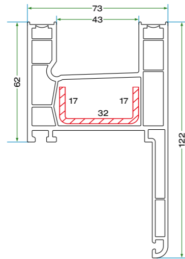
KPS 6207 PERVAZLI SÜRME KASA PROFİLİ KPS 6207 SLIDING FRAME PROFILE WITH BORDER
