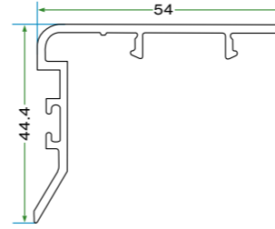
KPS 6203 İNEKLİLİKLİ KİLİT ADAPTÖRÜ KPS 6203 FLY SCREEN LOCK ADAPTER
