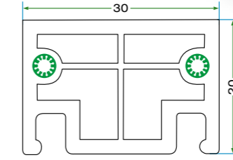
KPS 6205 SÜRME İNEKLİLİK ORTA KAYIT PROFİLİ KPS 6205 FLY SCREEN SLIDING MULLION PROFILE
